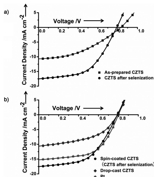
Figure 2. Photocurrent–voltage characteristics of DSSCs using CZTS or Pt films as CEs. a) As-prepared CZTS by spin coating but without sintering ( \blacksquare ) and spin-coated CZTS film after selenization (CZTSSe; \bullet ). b) Spin-coated CZTS film after selenization (CZTSSe; \bullet ), drop-cast CZTS film after selenization (CZTSSe; \blacklozenge ), and Pt film ( \star ).
